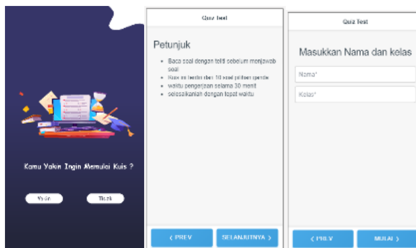
Figure 3. Quiz Menu
